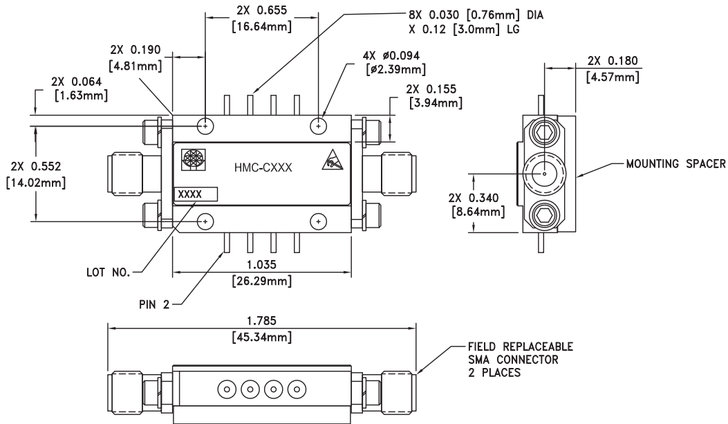
C-6 Package Outline Drawing
